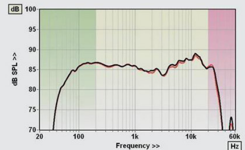
ABOVE: Response inc. nearfield summed driver/port [green], freefield corrected to 1m at 2.83V [yellow], ultrasonic [pink]. 'Left' speaker, black; 'right', red
